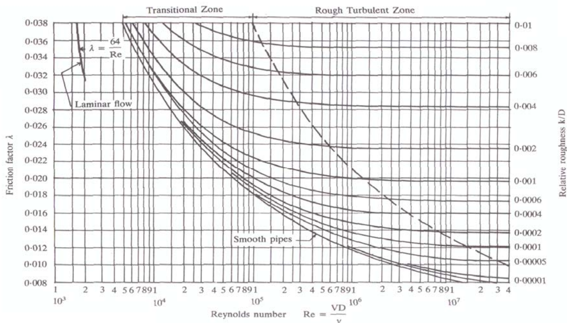
Moody Diagram
