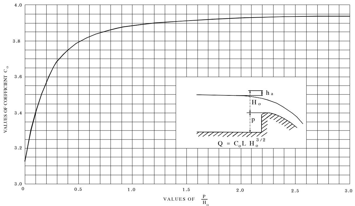
Discharge Coefficient for Vertical – faced Ogee Crest
