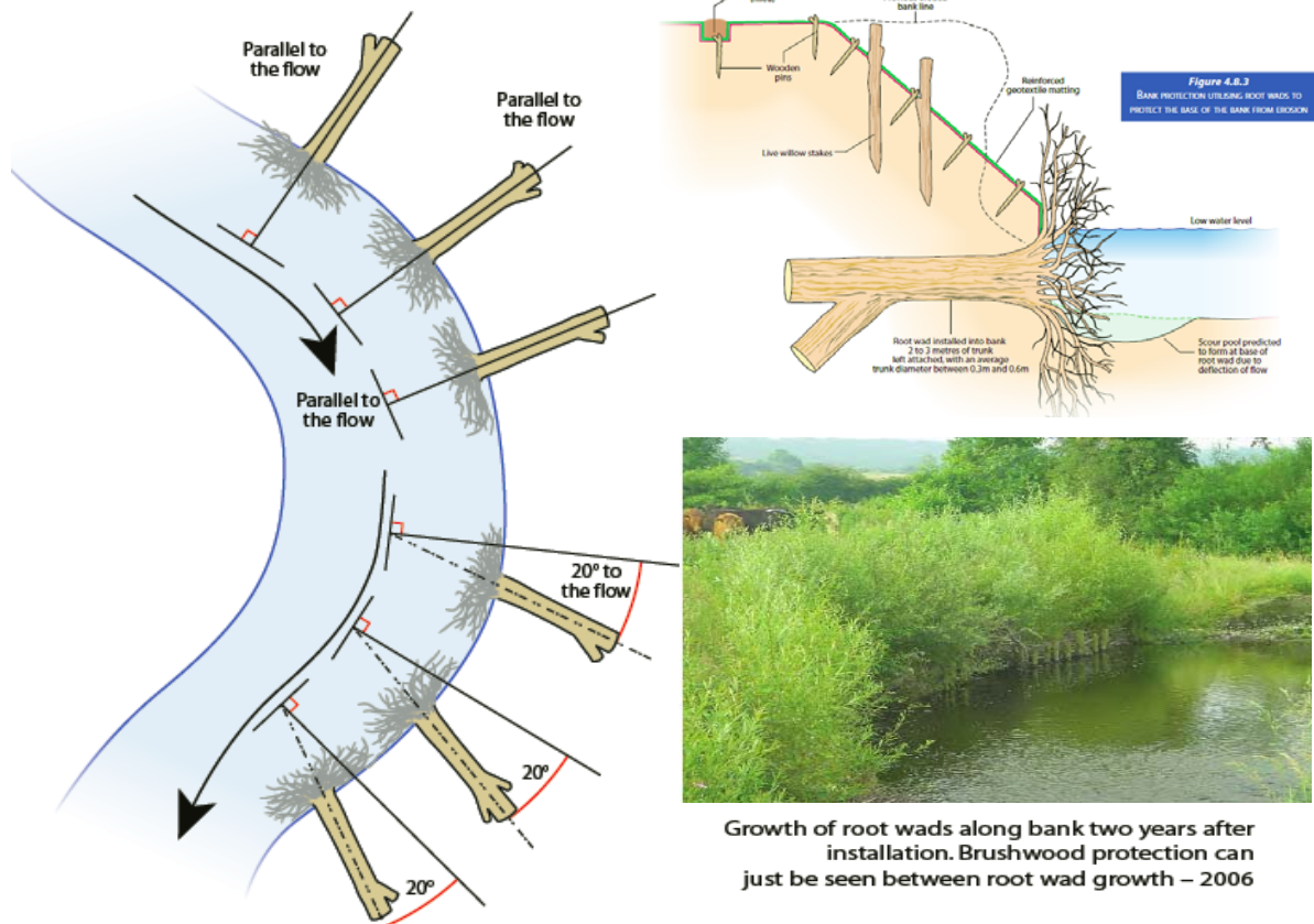
Bank protection using root wads
