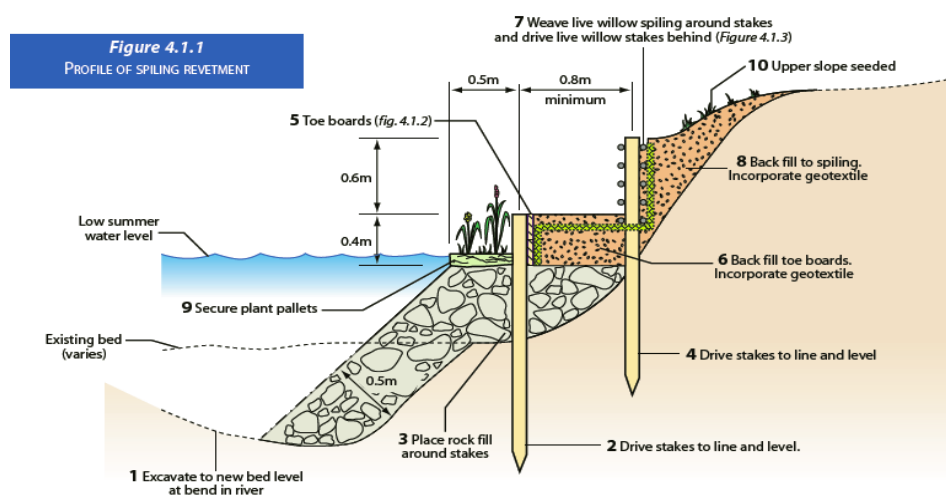
Willow mattress revetment
