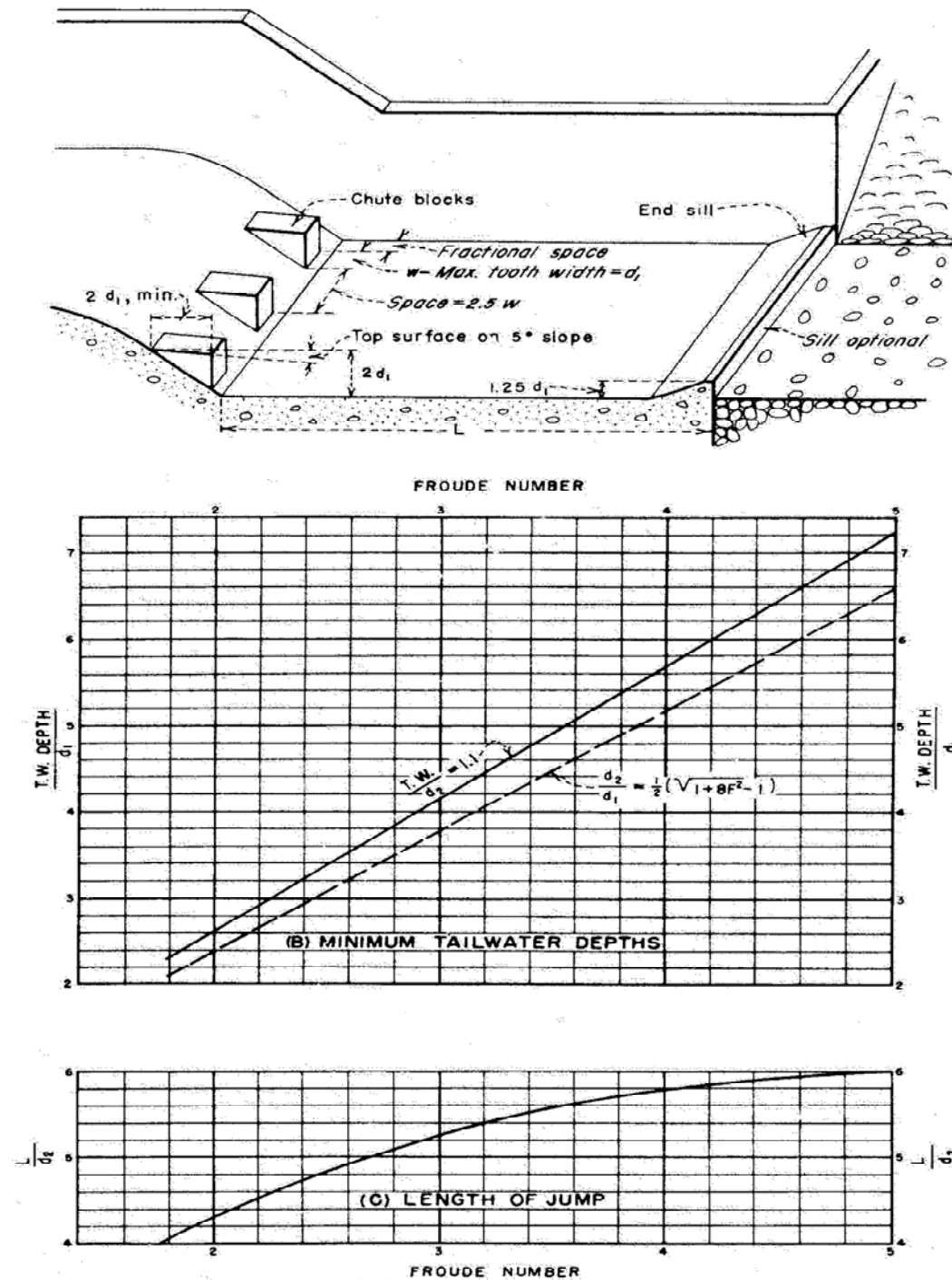
Stilling Basin Characteristics for Froude Number Between 2.5 and 4.5
